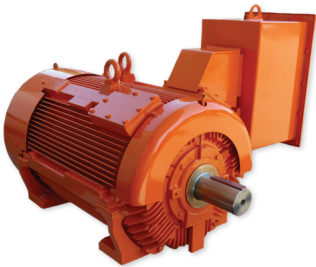
AFJE MAXe3 Mining Motor FRAME SIZES D315A-355
