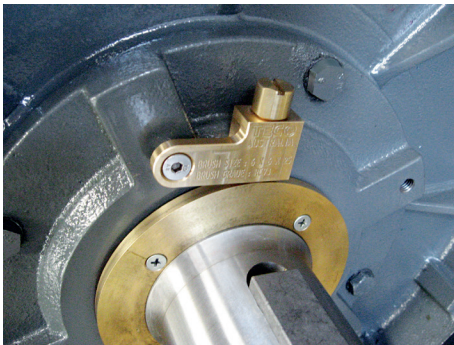
Rotor Grounding Brush fitted to a 280 Frame Motor.
