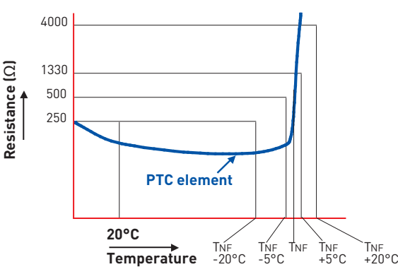
Temperature vs. Resistance Diagram
