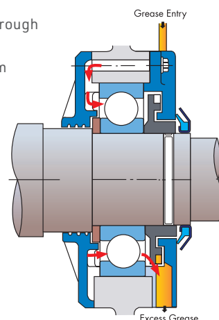
TECO Flush Through Grease Relief Bearing System with Brass Dust Flinger D280-355
