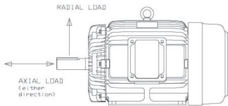
Axial Radial Loadings - Foot
