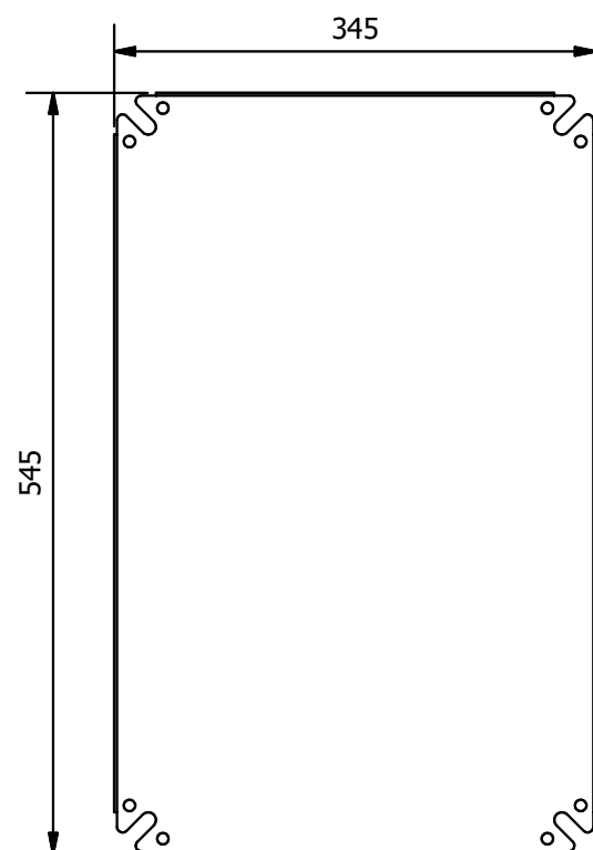
GEAR TRAY
