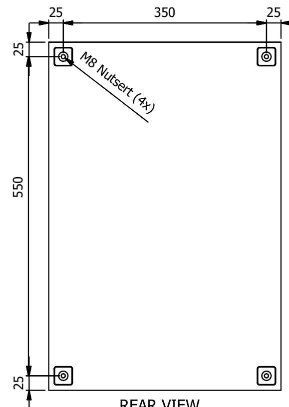
REAR VIEW
