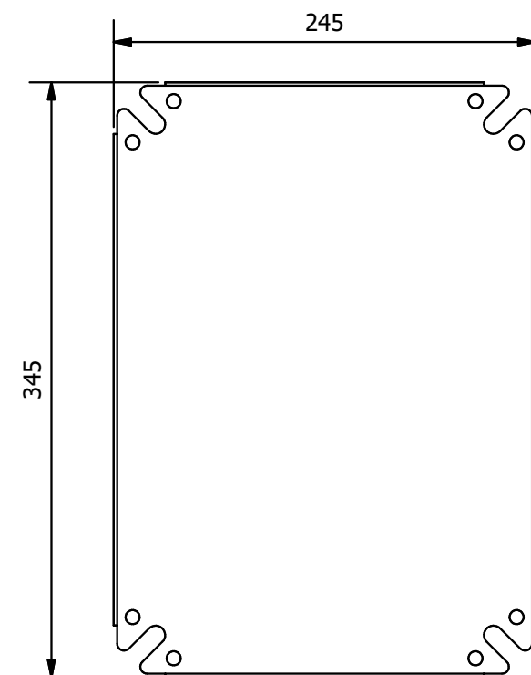
GEAR TRAY
