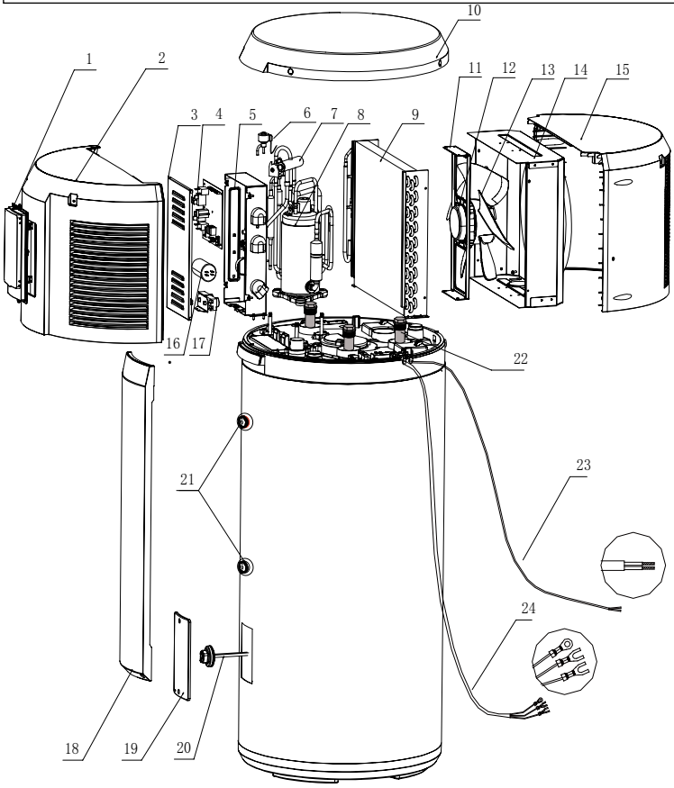
Exploded view of the heat pump
