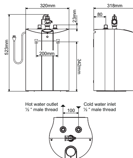
SHC 15 AU mains pressure compact storage water heater
