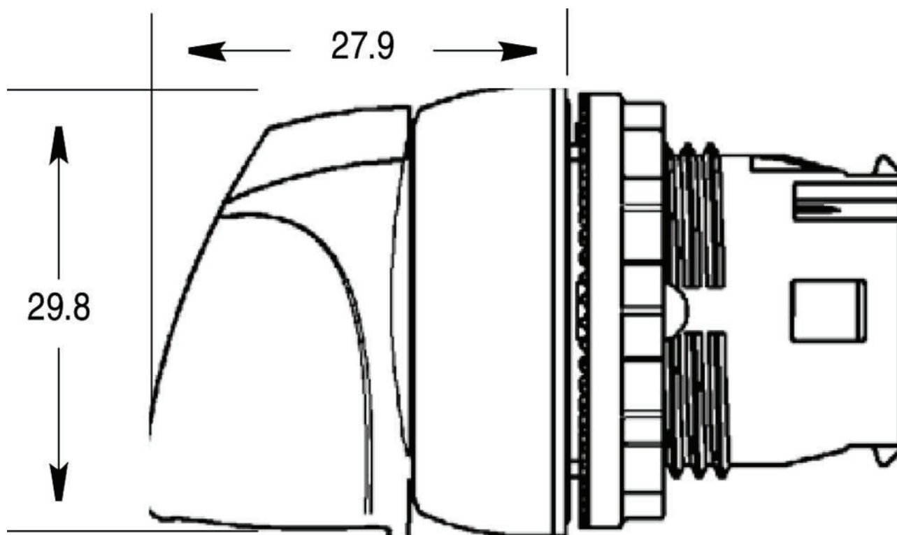
Dimension Diagram
