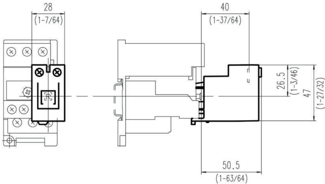
Dimension Diagram
