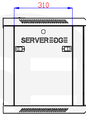
Side
