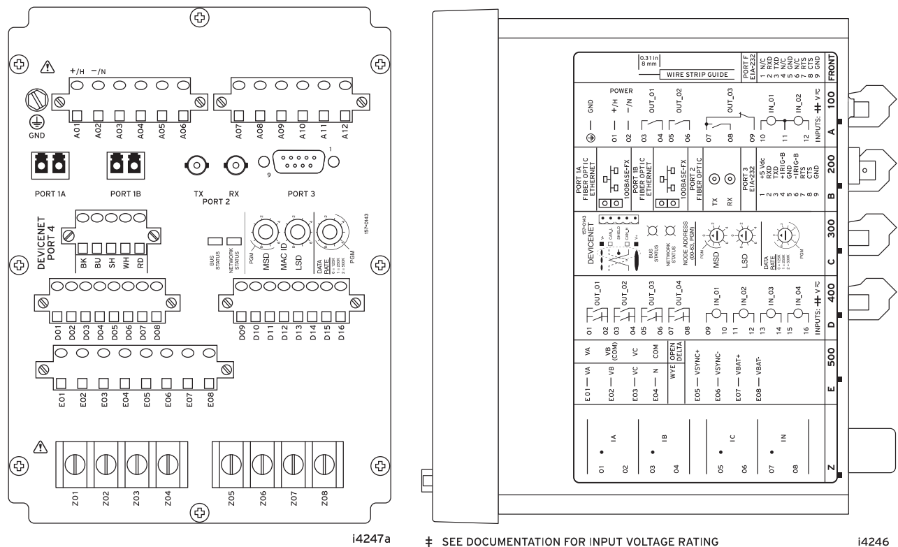
Figure 16 Dual Fiber Ethernet With Enhanced Voltage Option With Monitoring Package, DeviceNet, Fiber-Optic Serial Port, and Fast Hybrid 4 DI/4 DO
