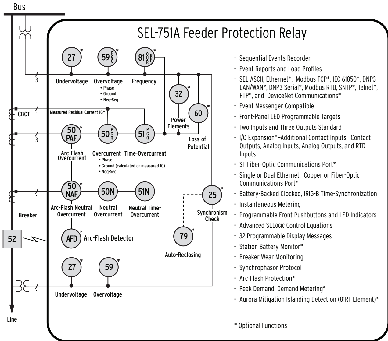
Figure 1 Functional Diagram
