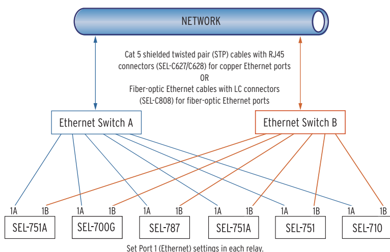
Figure 10 Ethernet Network Configuration With Dual Redundant Connections (Failover Mode)
