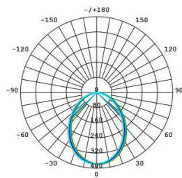
S9041 TC at 3000K
