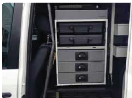
RC5/60 cabinet with 1 x RC602 & 1 x RC606 Dimensions: W - 600, D - 460, H - 547 (mm)
