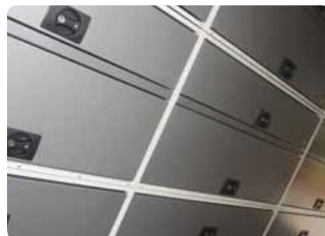
RC7/60 cabinet with 2 x RC603 & 2 x RC602 Dimensions: W - 600, D - 460, H - 743 (mm)
