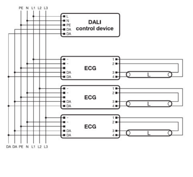
Wiring diagram
