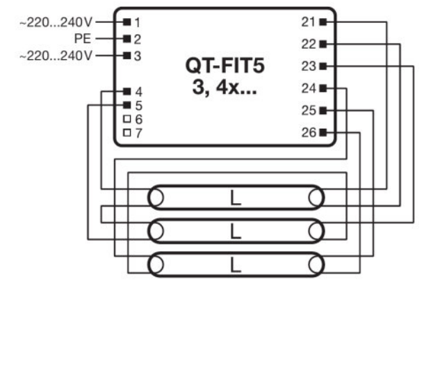
Wiring diagram
