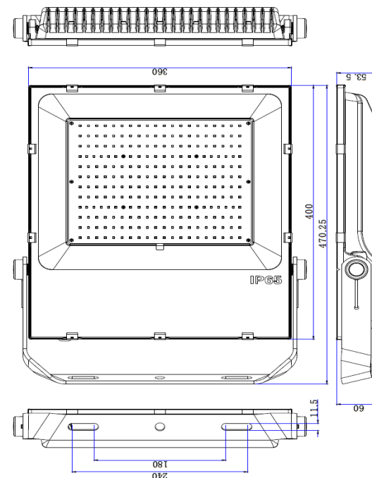
200w floodlight
