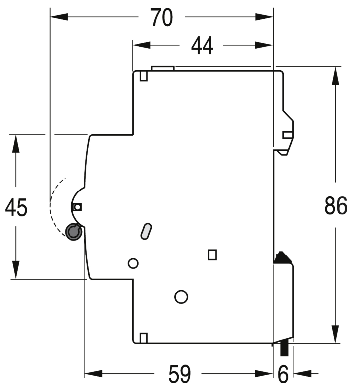
Dimension Diagram
