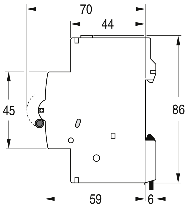
Dimension Diagram
