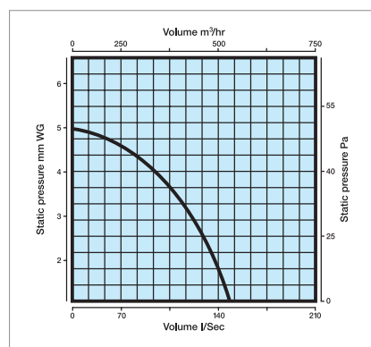
Performance - XFS230
