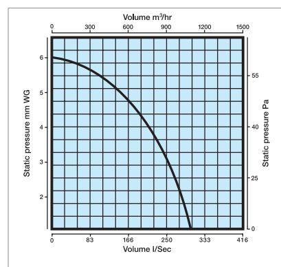
Performance - XFS300
