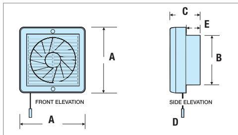
Dimensions - XF230/300
