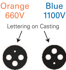
Colour and Orientation for Voltage
