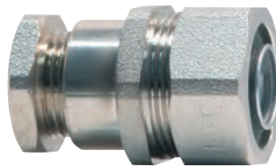
LC - SPS - B (IP66/67/68) Space Saver Multi part compression fitting with a nylon seal. Contains female threaded body component and a male threaded bush component, which minimises the amount of space taken up inside enclosures. Available in Brass (B)
