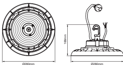
60W/80W/100W Ø280x166mm
