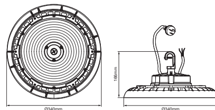
125W/150W/200W Ø343x166mm
