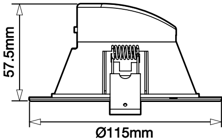
LDVAL DL SS 7.5W 90mm TRI G5 LED (4058075706217)
