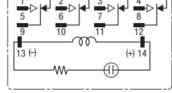
4PDT
