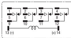
4PDT
