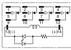
4PDT
