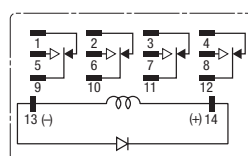
4PDT
