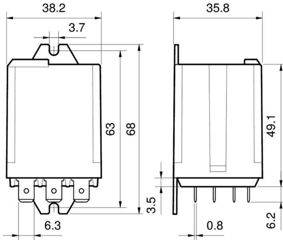
Dimension Diagram
