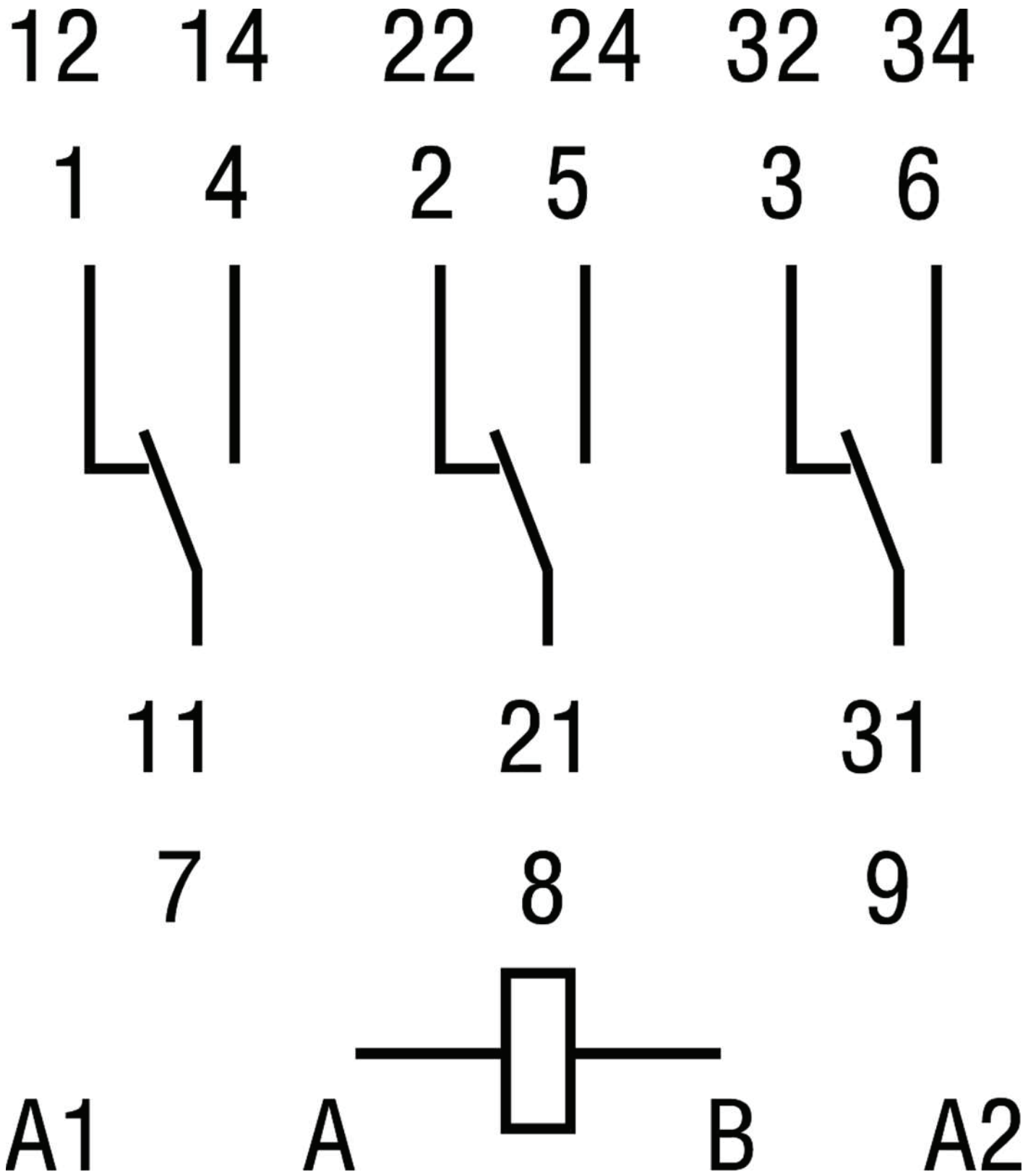
Connection / Wiring Diagram
