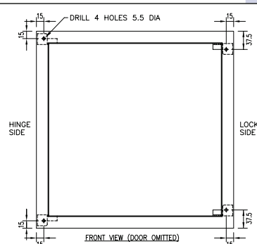
Drilling guide & bracket locations
