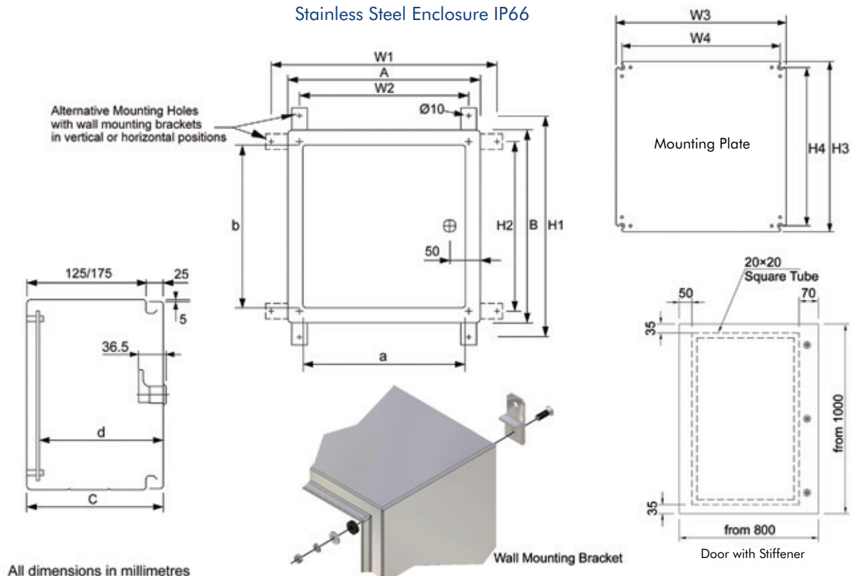
MAIN DIMENSIONS Stainless Steel Enclosure IP66
