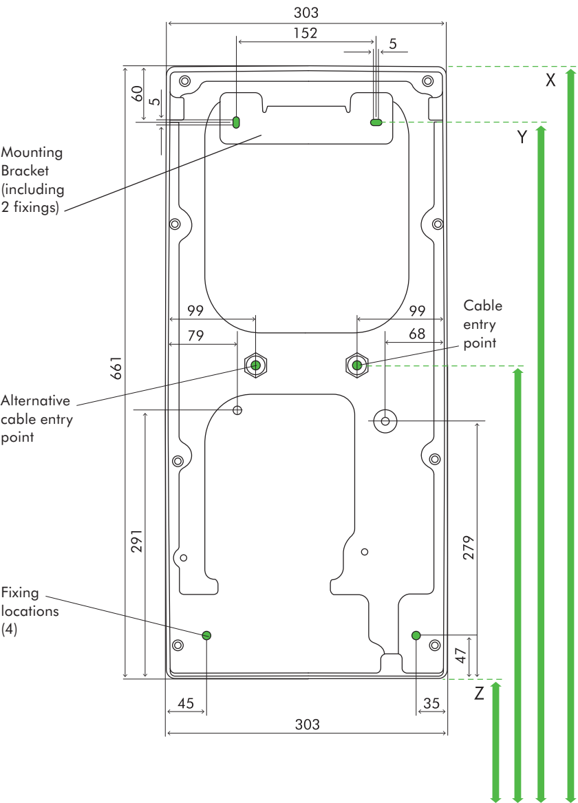
REAR ELEVATION
