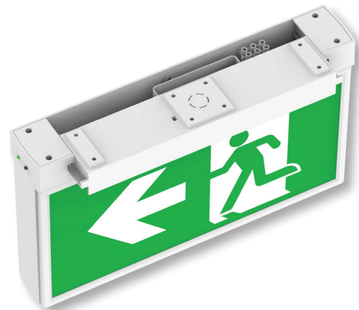
Slide-on control gear housing
