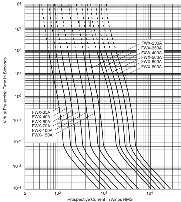
Time-Current Curve
