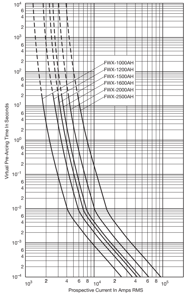
Time-Current Curve
