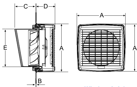
Window Axial
