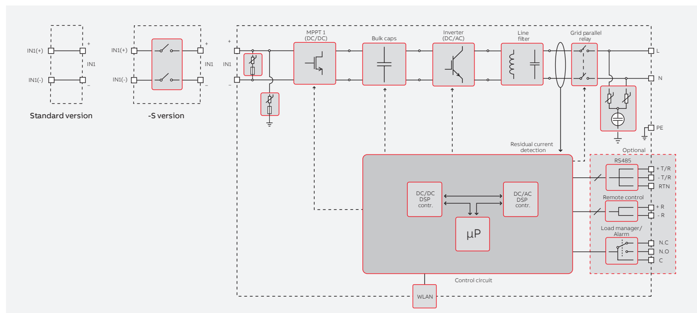
ABB UNO-DM-1.2/2.0/3.0-TL-PLUS-Q string inverter block diagram
