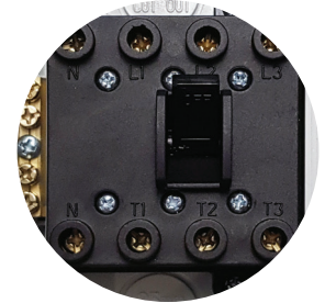
Example of internal 4-pole switch
